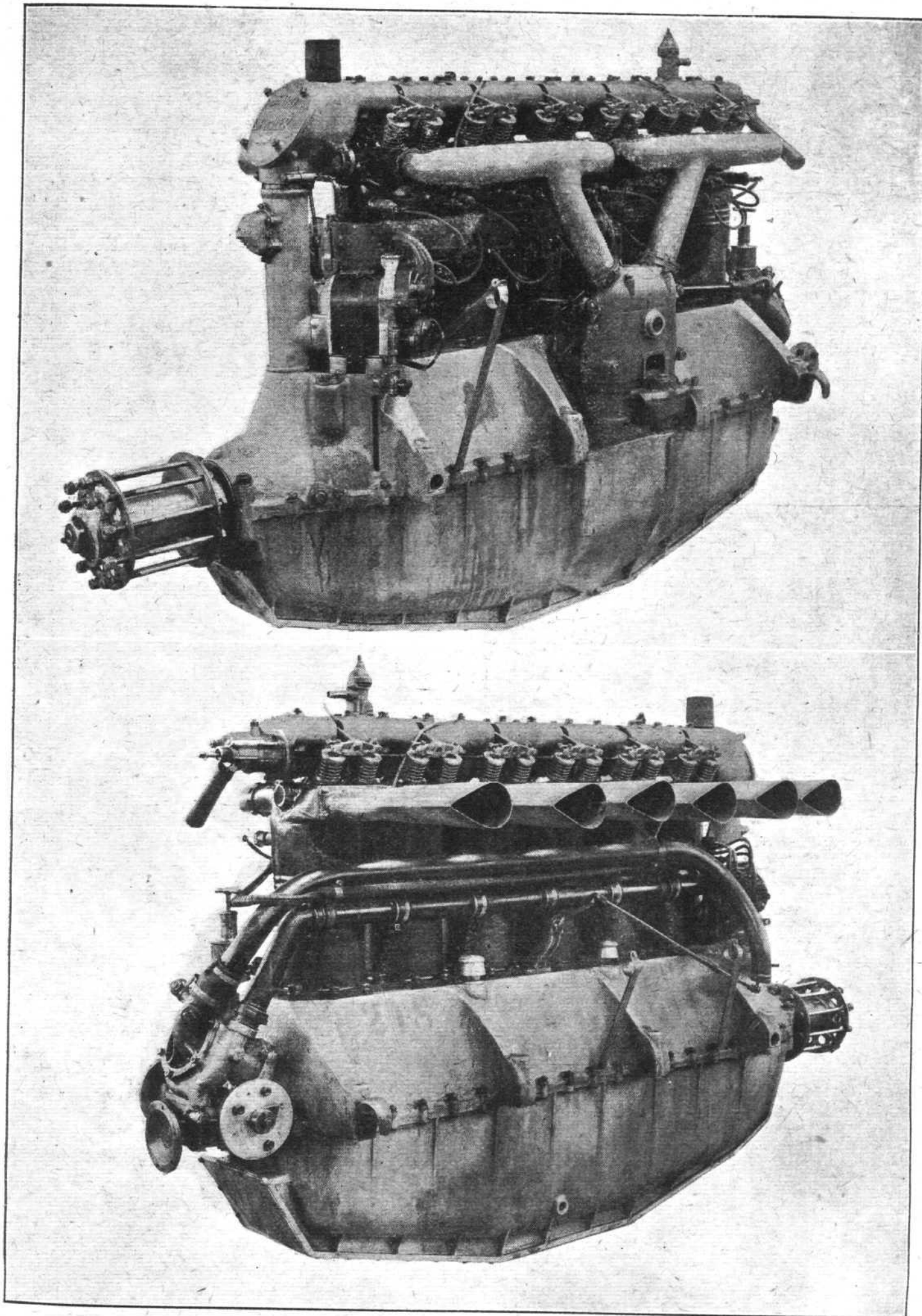
Top : Fig. 1.—The 200 h.p. Austro-Daimler engine. Induction side. Bottom : Fig. 2.—Exhaust side of engine. (See page 1218 and following pages.)
